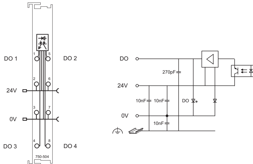
Fig. 2.1.1-3: 4-Channel Digital Output Module 750-504
